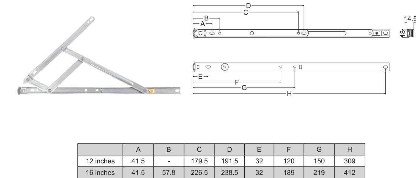
Easy-Clean Friction Hinges
