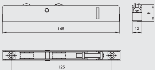
SL2IU0012009 (Carbon Steel Frame) SL2IU0012009.1 (SS304 Frame)
