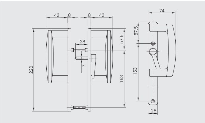
MSZ001825 L/R (H=25mm) MSZ002625 L/R (H=42mm)
