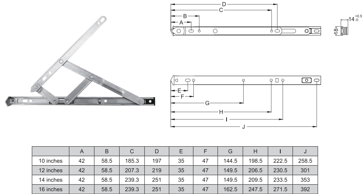
14mm Stack Height Friction Hinges
